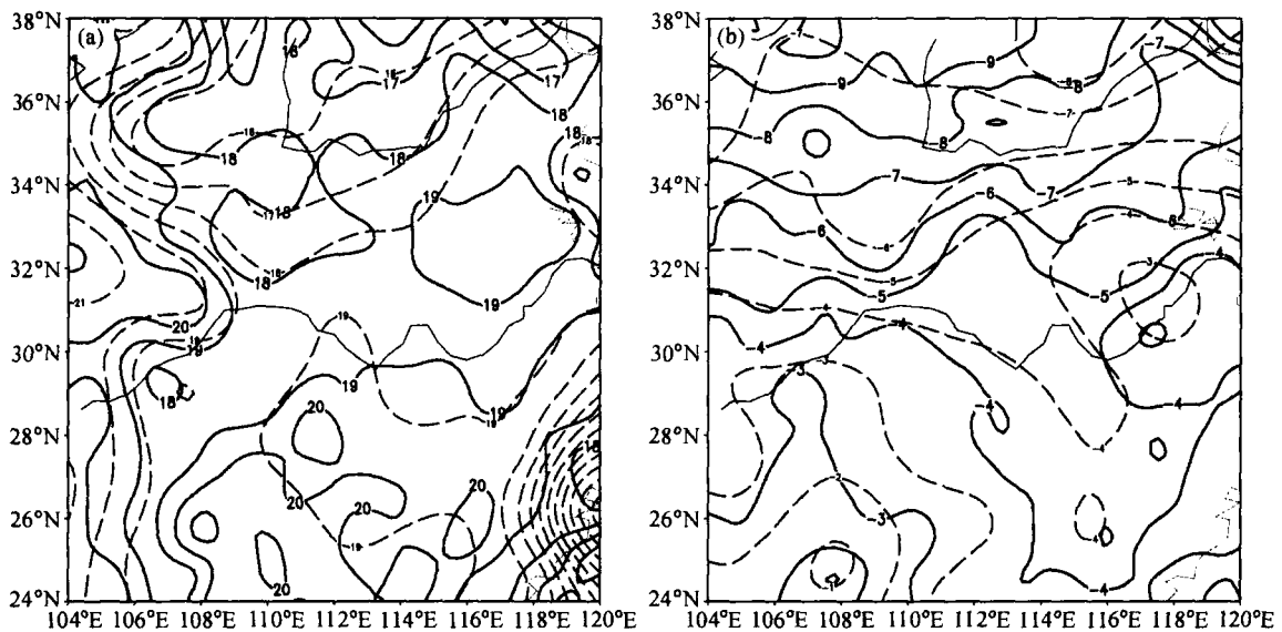
图 10 7 月 22 日 0000 UTC (a) 850 hPa、(b) 500 hPa 上 INDIRA TOVS 试验(实线)与 NOA TOVS 试验(虚线)温度分布(单位: ) Fig. 10 The temperature (units: ) at (a) 850 hPa and (b) 500 hPa at 0000 UTC 22 Jul 2002 in INDIRA TOVS (solid line) and NOA TOVS (dashed line)
