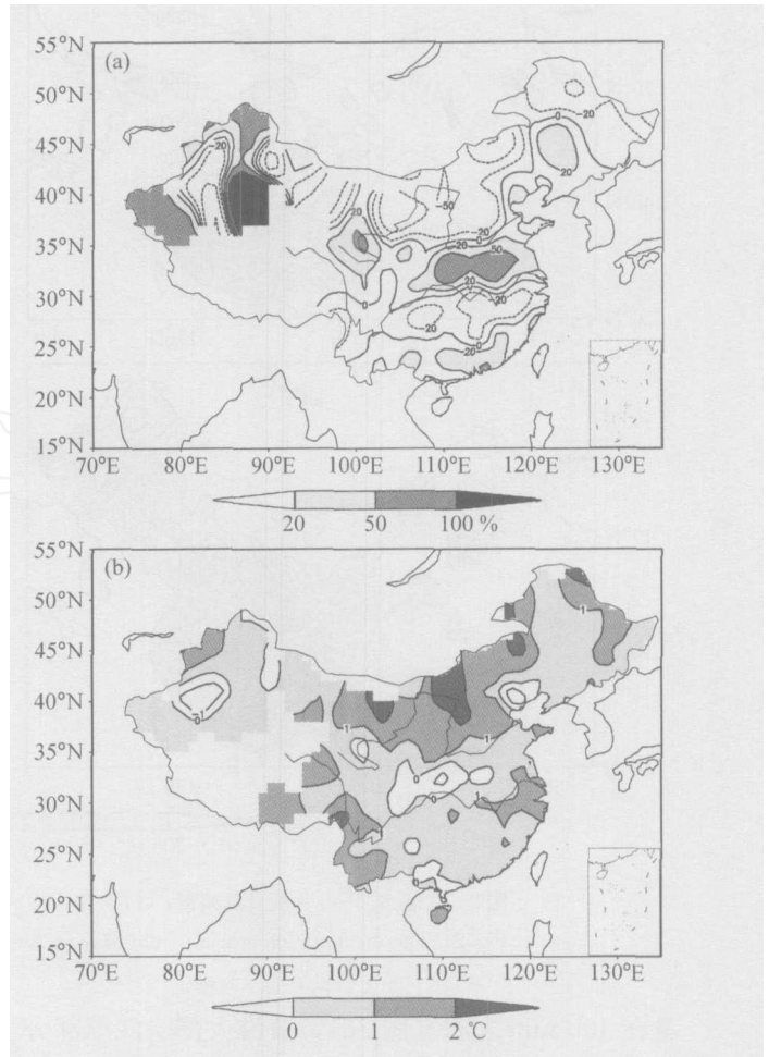
图 1 2005 年 6~8 月中国降水距平百分率 (a) 与气温距平 (b) Fig. 1 The percentage anomaly of precipitation amount (a) and temperature anomaly (b) from the average from June to August 2005
