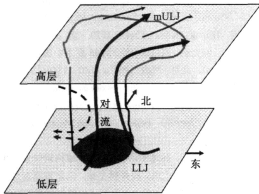
图3 “96.8”暴雨的中尺度对流系统模型(引自文献[70]) Fig. 3 The schematic model of the mesoscale convective system of torrential rain in Aug 1996 (from reference [70])
