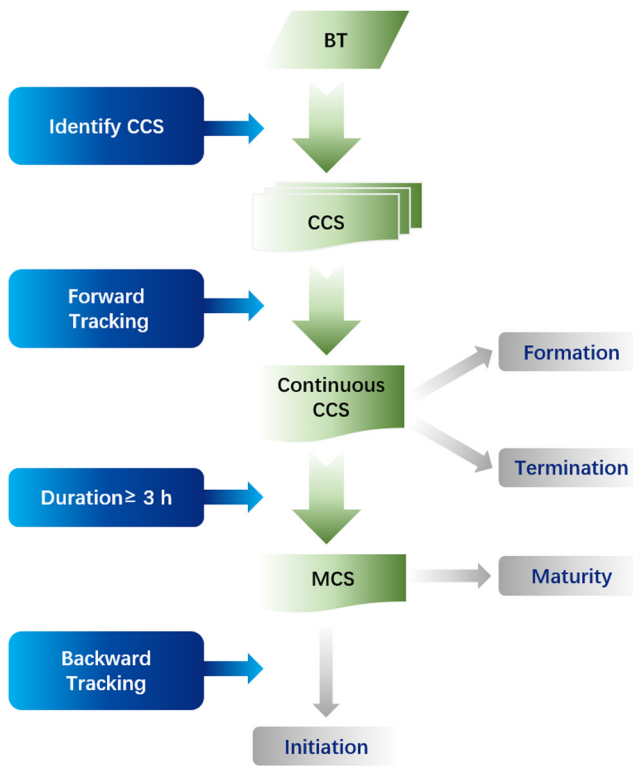
Figure 2. Flow chart of mesoscale convective system (MCS) identification and tracking.
