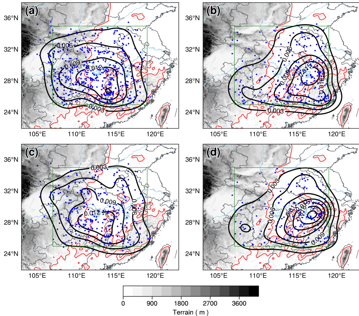
Figure 5. The spatial distribution of initiation locations of quasistationary (QS) mesoscale convective systems (MCSs) during the entire warm season (a) and in July and August (c) and outward-moving (OM) MCSs during the entire warm season (b) and in June and July (d). The blue dots represent initiation locations, from which the spatial probability density is calculated and exhibited by the black contours. The green rectangle marks the middle reaches of the Yangtze River Basin. The gray shading represents terrain height (m) and the red contours denote the terrain height of 300 m.
