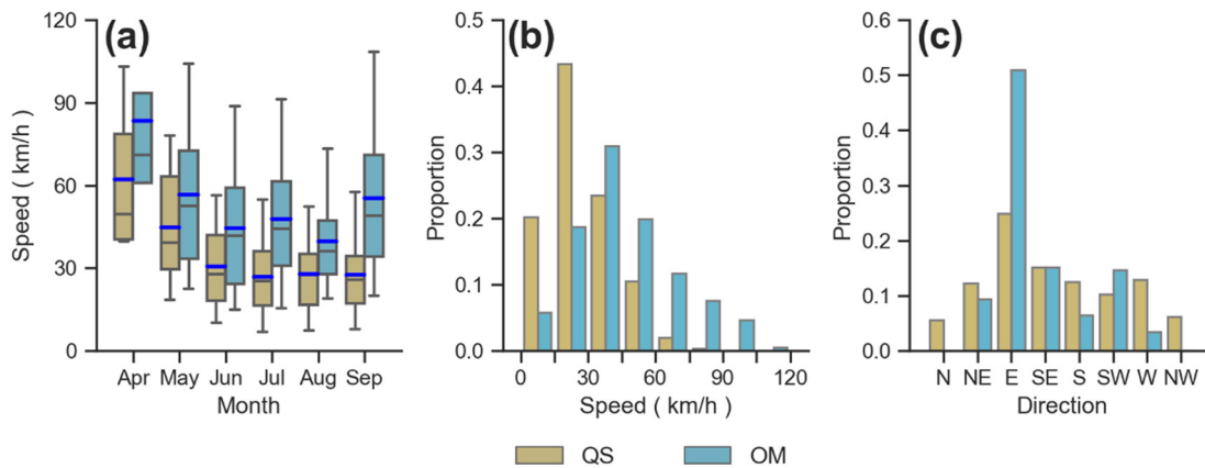
Figure 6. Box-and-whisker plot of mesoscale convective system (MCS) speed (a, \text{km h}^{-1} ) during the warm seasons of 2018–2021 (a). The upper and lower edges (caps) of the boxes (whiskers) in the box-and-whisker plot represent the third and first quartiles (95th and 5th percentiles), respectively. The black (blue) dashes inside the boxes represent the medians (mean values). Histograms of MCS movement speeds (b, \text{km h}^{-1} ) and directions (c) in the high occurrence period.
