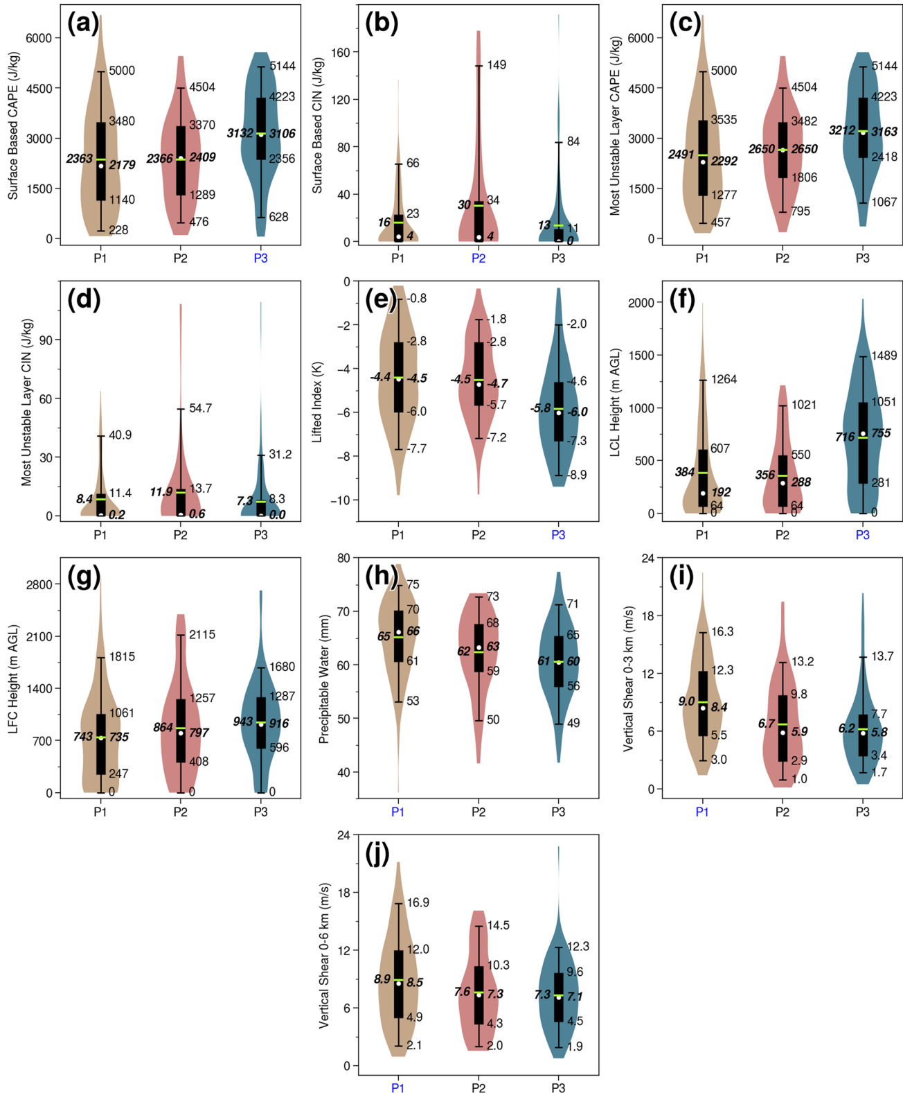
Figure 10. Violin plots of environmental parameters. From (a) to (j) are SBCAPE ( J kg^{-1} ), SBCIN ( J kg^{-1} ), MUCAPE ( J kg^{-1} ), MUCIN ( J kg^{-1} ), LI (K), LCL (m), LFC (m), PW (mm), SHR3 ( m s^{-1} ), and SHR6 ( m s^{-1} ). The outline of the violin represents the probability density. The upper and lower edges (caps) of the box (whiskers) inside the violin represent the third and first quartiles (95th and 5th percentiles), respectively, which are marked on the right side of the violin. The white dot (lemon dash) inside the box represents the median (mean value), which is marked in bold italics on the right (left). The pattern label marked blue indicates that the mean value of the parameter in this pattern is significantly (above the 95% level based on a two-tailed Welch's t test) different from those in the other two patterns.
