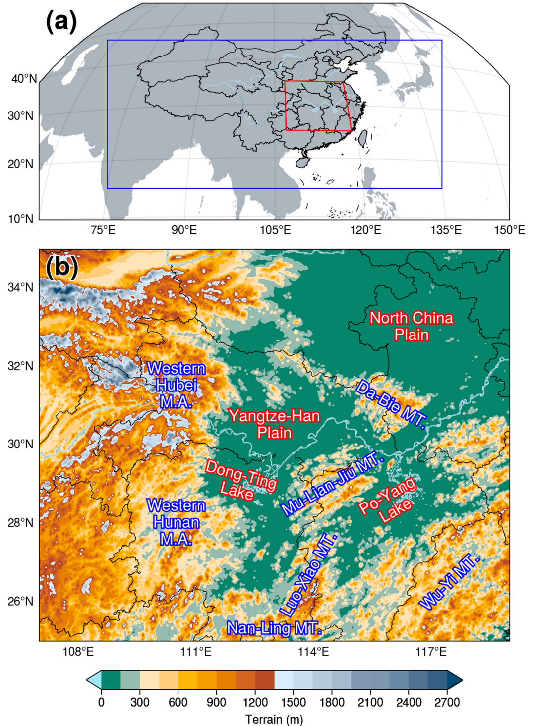
Figure 1. (a) The coverage of brightness temperature data (blue rectangle) in the present study and the boundary of the middle reaches of the Yangtze River Basin (YRB) (red line). (b) The terrain height (m) in the middle reaches of the YRB. Mountains (MT.) and mountain areas (M.A.) are labeled in blue, and plains and lakes are labeled in red.
