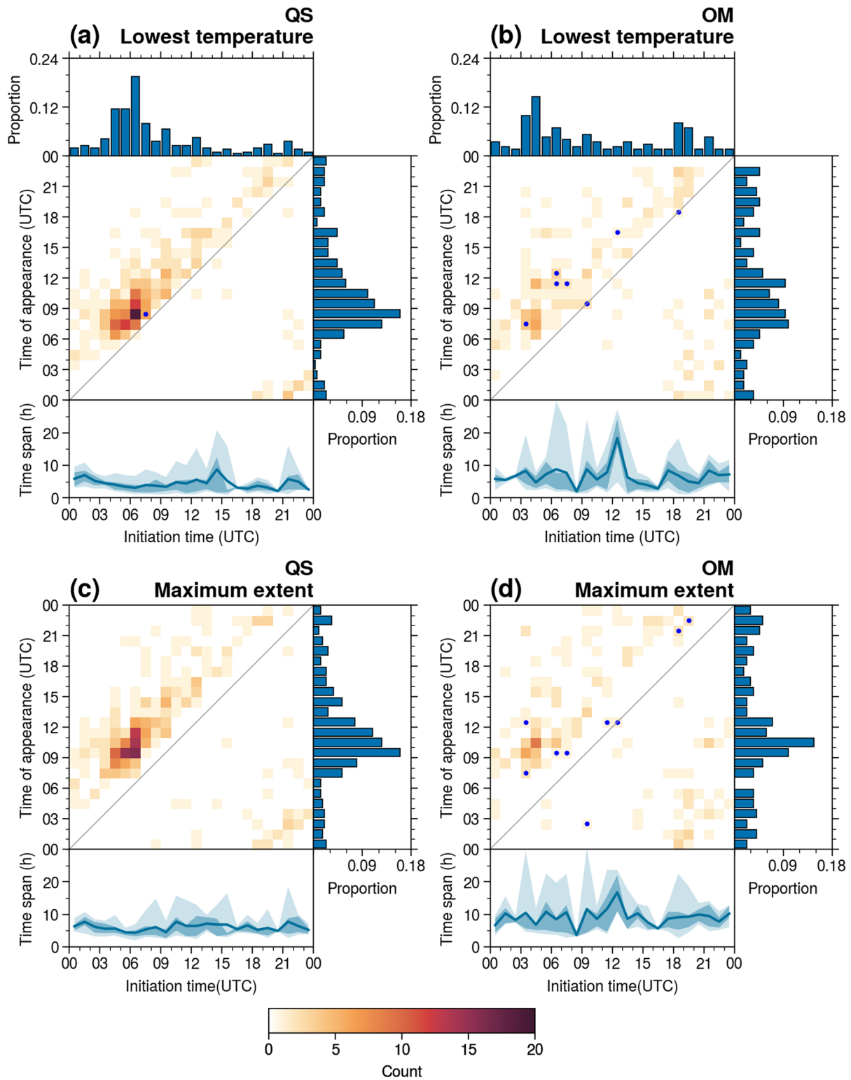
Figure 8. The two-dimensional histogram for the diurnal variation in the lowest temperature appearance of quasistationary (QS) mesoscale convective systems (MCSs) (a) and outward-moving (OM) MCSs (b) and the maximum extent appearance of QS MCSs (c) and OM MCSs (d) in the high occurrence period of 2018–2021. The main body of each plot exhibits the frequency of MCS initiation and the lowest temperature (maximum extent) in every hourly interval. The upper histogram exhibits the proportion of MCS initiation. The left histogram exhibits the proportion of the lowest temperature (maximum extent) appearance. The lower plot exhibits the time span between the lowest temperature (maximum extent) appearance and MCS initiation, with the solid line representing the mean time span and the light (dark) shading representing the 5%–95% (25%–75%) percentile interval. The blue dot indicates that the time span is longer than 24 hr.
