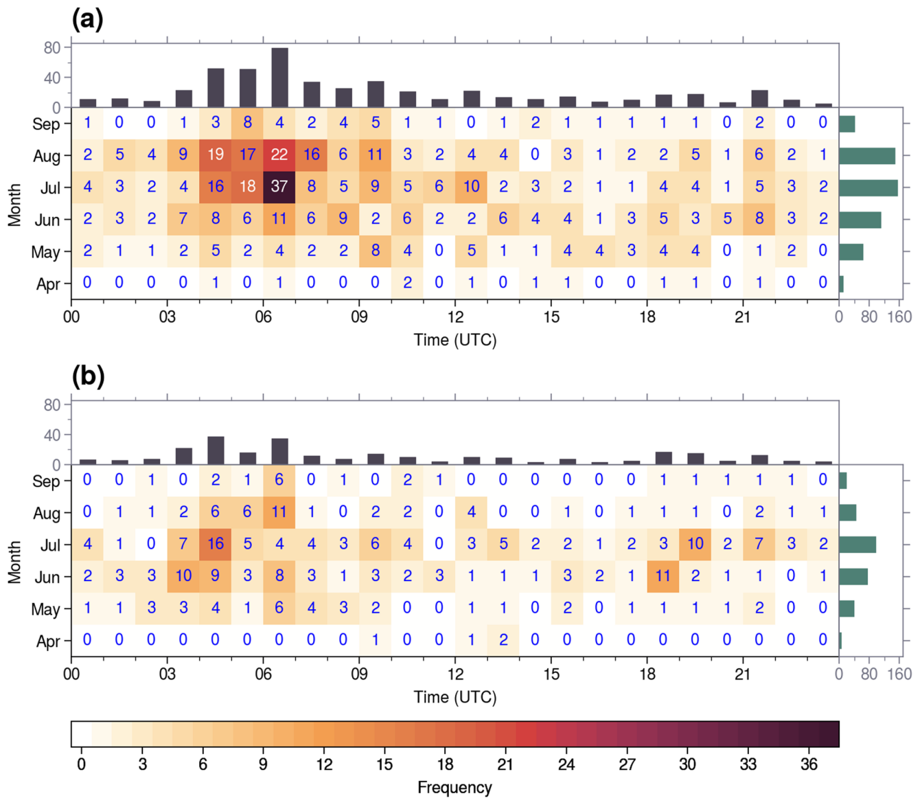
Figure 4. Monthly and diurnal distributions of the quasistationary (QS) mesoscale convective system (MCS) frequency (a) and the outward-moving (OM) MCS frequency (b) in the middle reaches of the Yangtze River Basin during the warm seasons (April–September) of 2018–2021. The horizontal axis represents the initiation time (UTC). The color shading symbolizes the occurrence frequency of MCSs.
