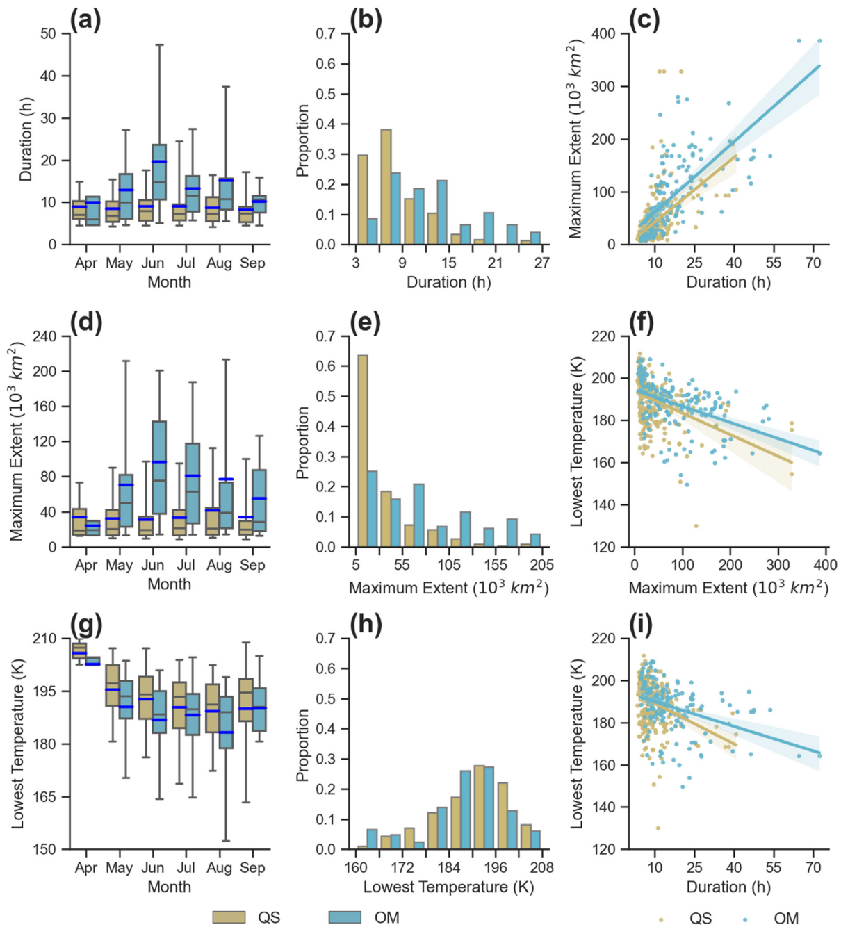
Figure 7. The box-and-whisker plots on the left are the duration (a), the maximum extent (d), and the lowest temperature (g) of mesoscale convective systems (MCSs) during the entire warm season of 2018–2021. The upper and lower edges (caps) of the boxes (whiskers) in the box-and-whisker plot represent the third and first quartiles (95th and 5th percentiles), respectively. The black (blue) dashes inside the boxes represent the medians (mean values). The histograms of the central column are the proportion of the duration (b), the maximum extent (e), and the lowest temperature (h) of MCSs in high occurrence periods of 2018–2021. The scatter plots on the right are the pairwise relationships between the duration and the maximum extent (c), the maximum extent and the lowest temperature (f), and the duration and the lowest temperature (i) in high occurrence periods of 2018–2021.
