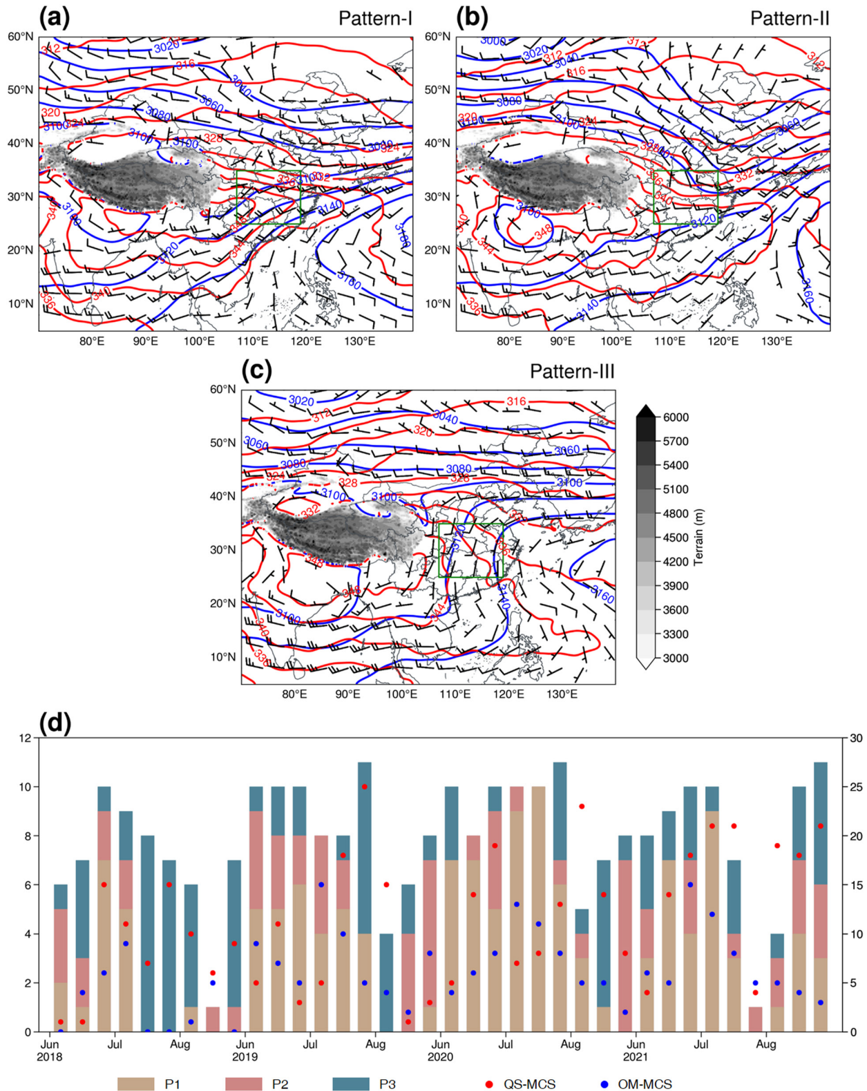
Figure 9. The composite geopotential fields (blue contours, gpm), equivalent potential temperature fields (red contours, K), and wind fields (wind barbs, m s^{-1} ) at 700 hPa of P1 (a), P2 (b), and P3 (c), respectively. A half (full) barb represents 2 m s^{-1} ( 4 m s^{-1} ). The green rectangle marks the middle reaches of the Yangtze River Basin. The gray shading represents terrain heights (m). The bars (scatters) in (d) represent the occurrence frequency of three circulation patterns (two types of mesoscale convective systems [MCSs]) over each 10-day period from June to August of 2018–2021, corresponding to the left (right) vertical axis. Note that for July and August, the last 10-day period has 11 days.
