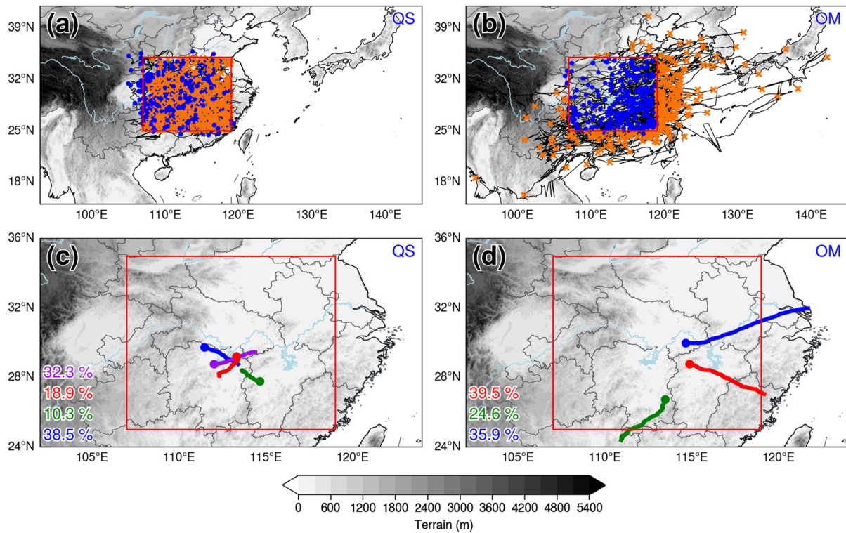
Figure 3. The movement trajectories of quasistationary (QS) mesoscale convective systems (MCSs) (a) and outward-moving (OM) MCSs (b) and the composite movement paths of QS MCSs (c) and OM MCSs (d). The blue dots (orange crosses) in (a) and (b) represent the initiation (termination) locations of MCSs. Different kinds of paths are distinguished by different colors in (c) and (d), and the proportions of trajectories in different kinds are marked in the lower left corner. The gray shading represents terrain height (m). The red rectangle indicates the boundary of the middle reaches of the Yangtze River Basin.
